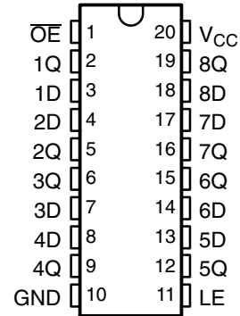
SN54AC373 . . . J OR W PACKAGE SN74AC373 . . . DB, DW, N, NS, OR PW PACKAGE (TOP VIEW)
