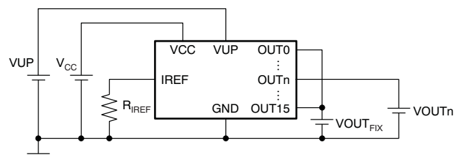
Figure 10. Leakage Current of Pre-Charge FET Test Circuit for OUTn
