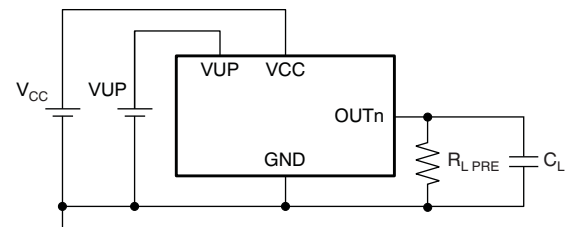
Figure 8. Delay Time Test Circuit for Pre-Charge FET
