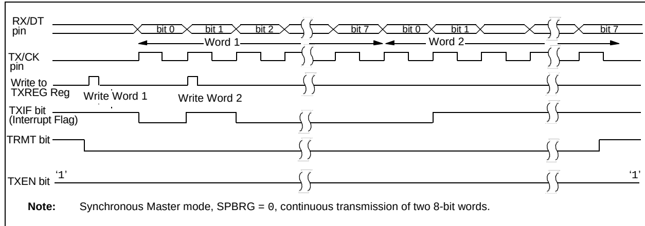
FIGURE 16-6: SYNCHRONOUS TRANSMISSION
