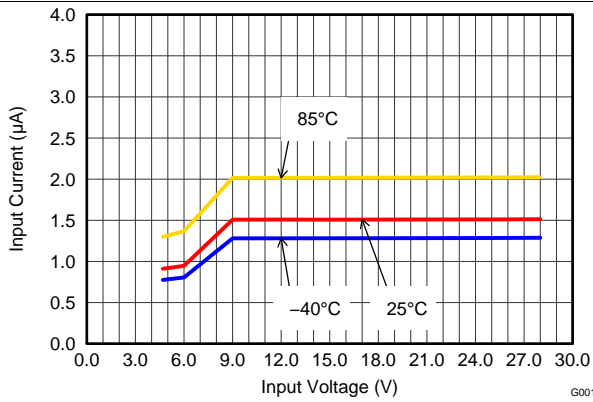
Figure 1. Quiescent Current
