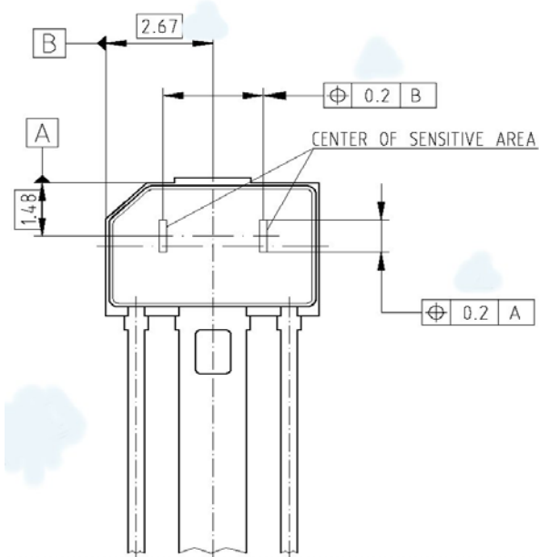
Figure 18 Package Dimensions (PG-SSO-3-6)
