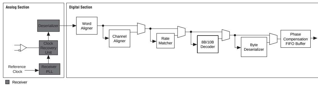
Figure 2–7. Highlighted Block Diagram of the Receiver Analog Components
