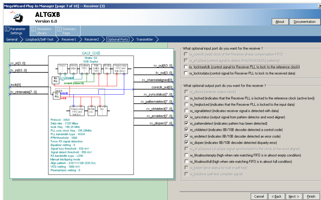
Figure 5–32. MegaWizard Plug-In Manager - altqxb (Page 7)
