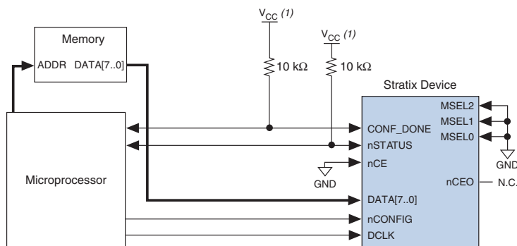
Figure 1–12. Parallel Configuration Using a Microprocessor
