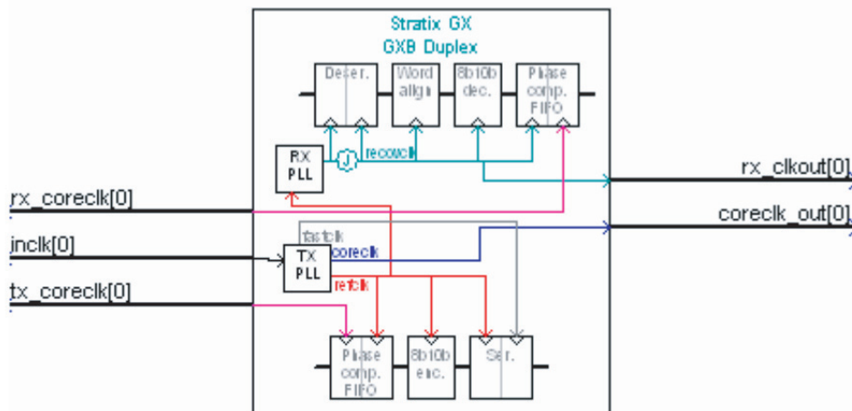
Figure 3–21. altgxb in Custom Mode With rx_coreclk &amp; tx_coreclk Enabled
