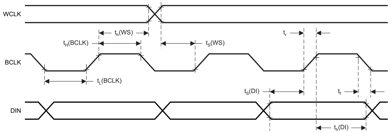
Figure 2. I 2 S/LJF/RJF Timing in Slave Mode
