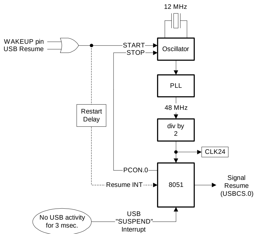
Figure 11-1. Suspend-Resume Control
