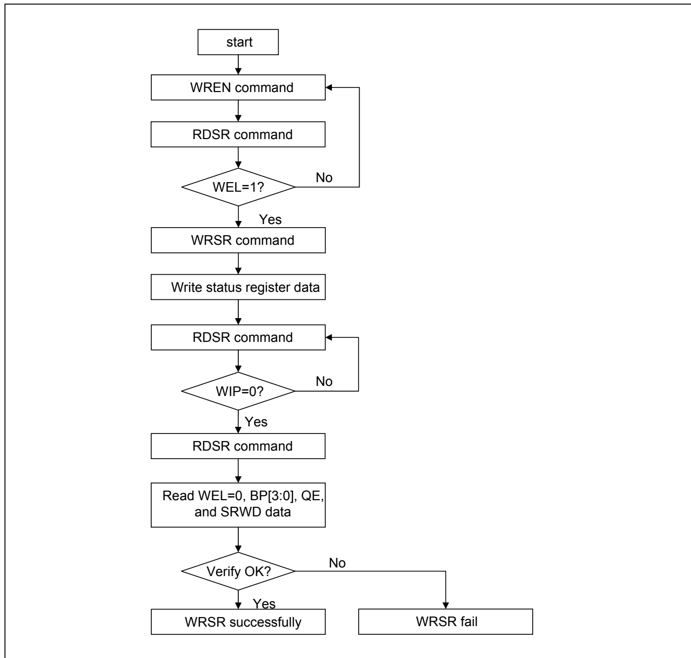
Figure 25. WRSR flow
