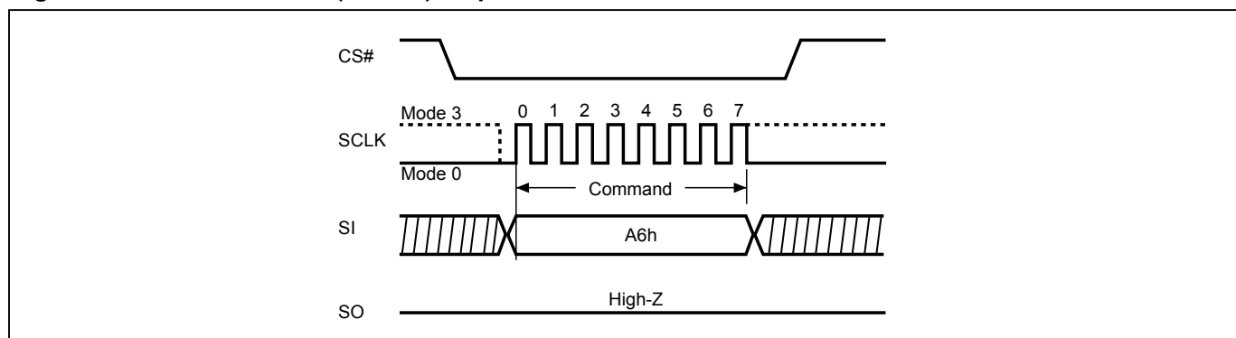
Figure 64. SPB Lock Bit Set (SPBLK) Sequence
