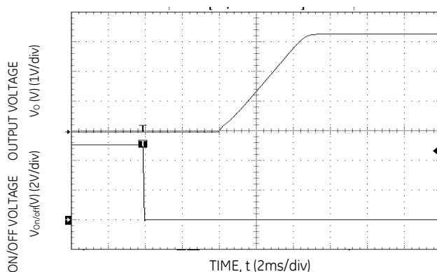
Figure 15. Typical Start-Up Using Remote On/Off with Low-ESR external capacitors (7x150uF Polymer) ( V_{in} = 5.0\text{Vdc} , V_o = 3.3\text{Vdc} , I_o = 3\text{A} , C_o = 1050\text{ }\mu\text{F} ).
