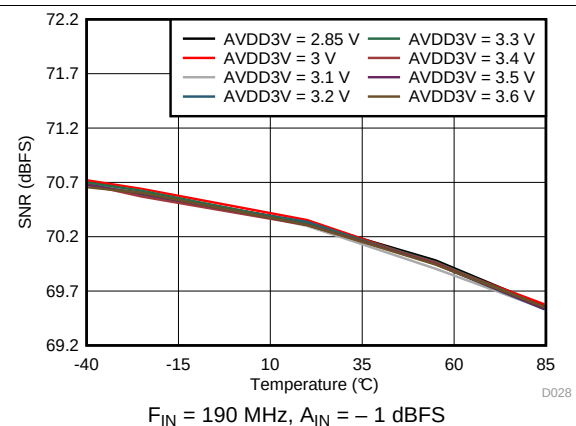
Figure 29. Signal-to-Noise Ratio vs AVDD3V Supply and Temperature
