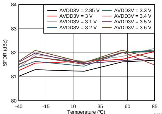
Figure 32. Spurious-Free Dynamic Range vs AVDD3V Supply and Temperature
