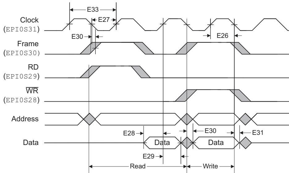
Figure 5-29. General-Purpose Mode Read and Write Timing
