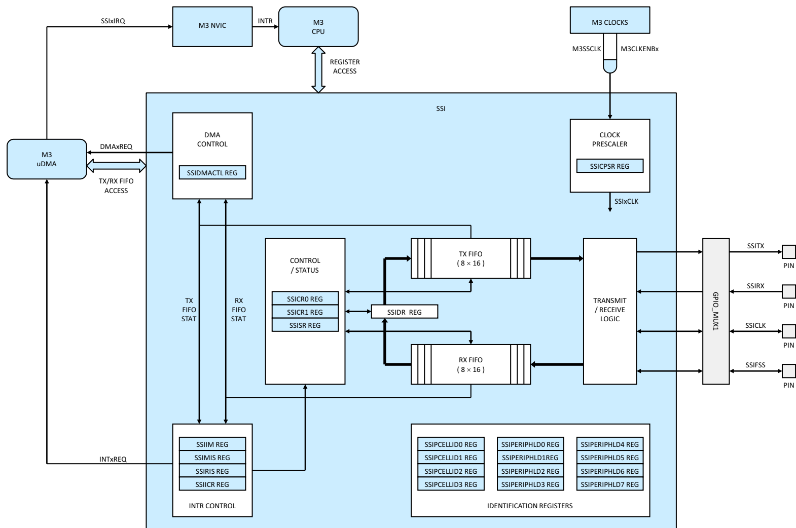
Figure 5-31. SSI
