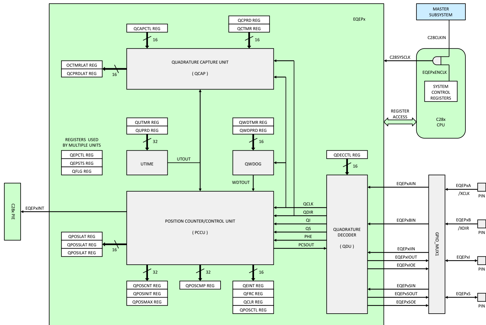
Figure 5-48. eQEP
