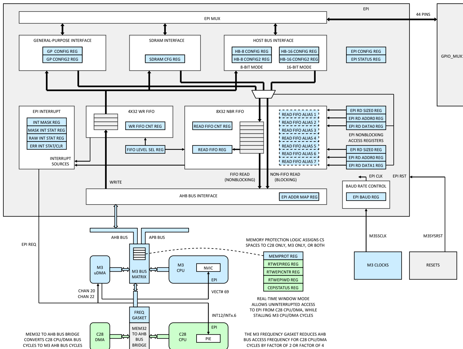
Figure 5-17. EPI
