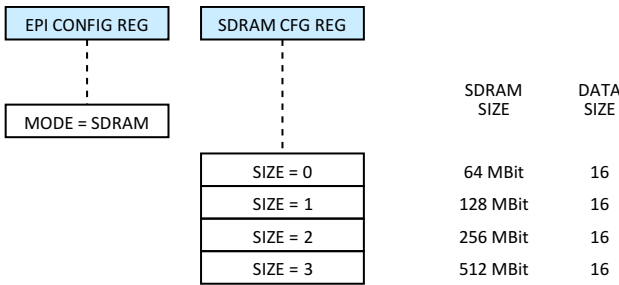
Figure 5-19. EPI SDRAM Mode
