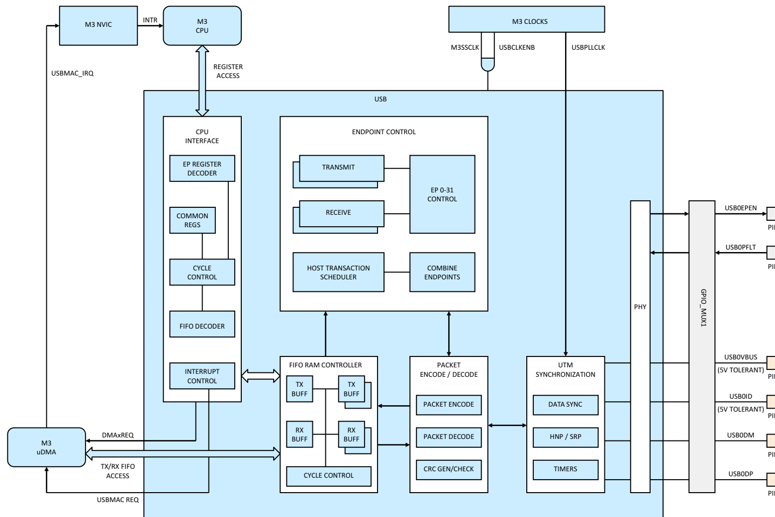
Figure 5-35. USB
