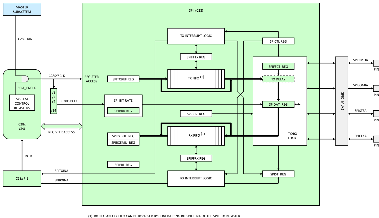
Figure 5-51. SPI (C28x)
