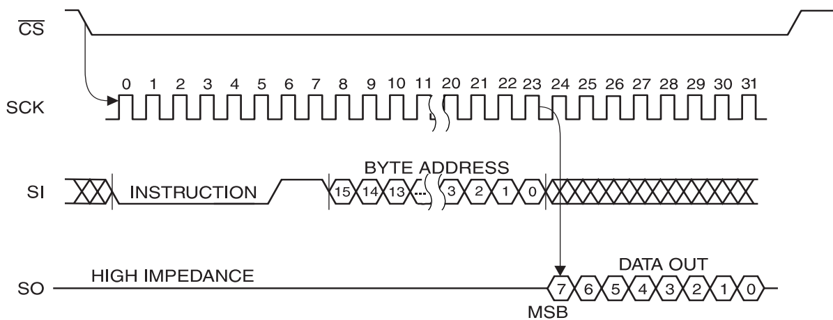
Figure 8. READ Timing
