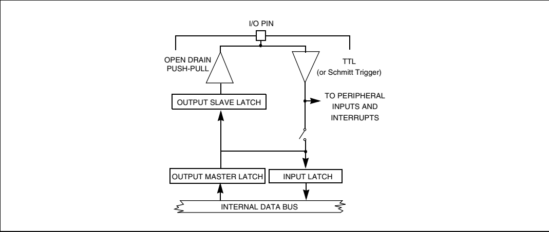
Figure 81. Output configuration
