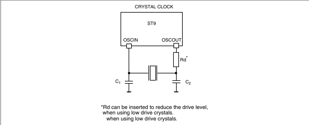
Figure 66. Crystal oscillator
