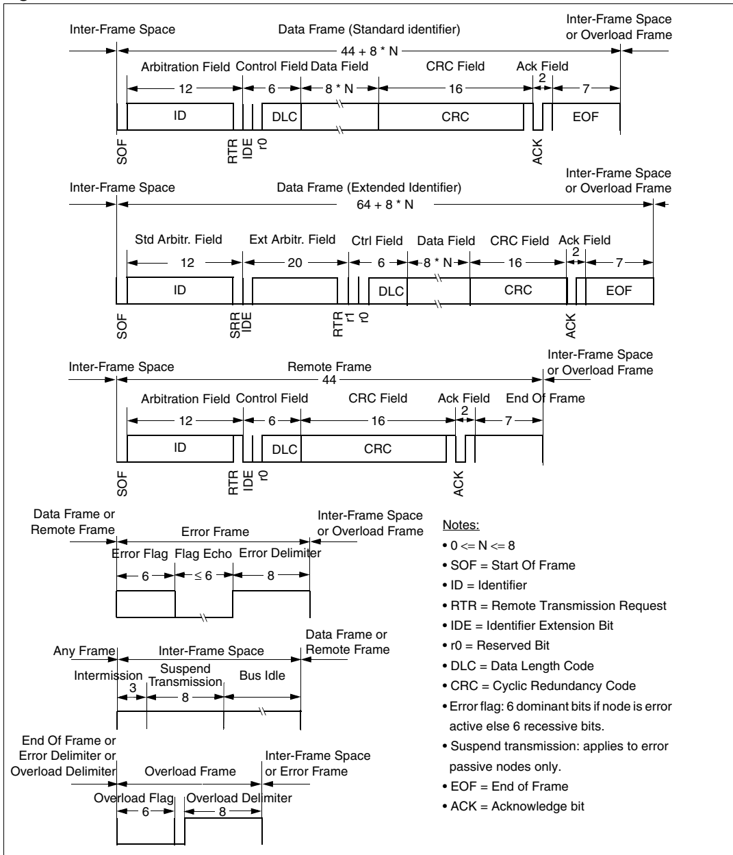
Figure 167. CAN frames
