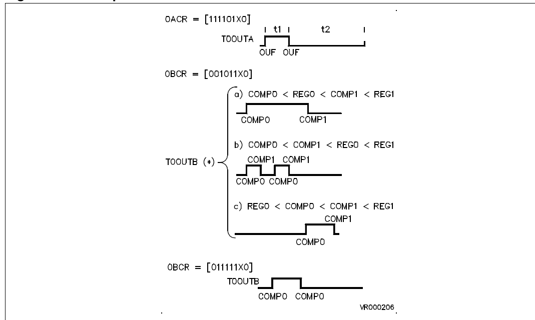
Figure 118. Sample waveforms
