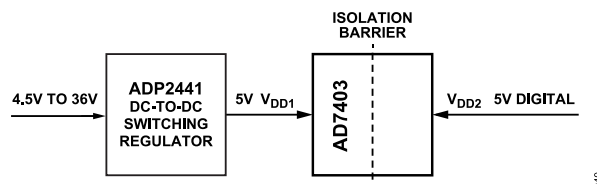
Figure 42. ADP2441 Step-Down DC-to-DC Regulator Example
