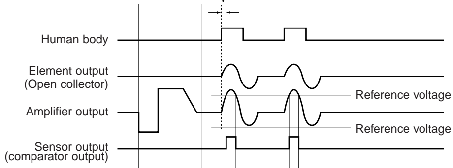
<Timing chart> Standard type
