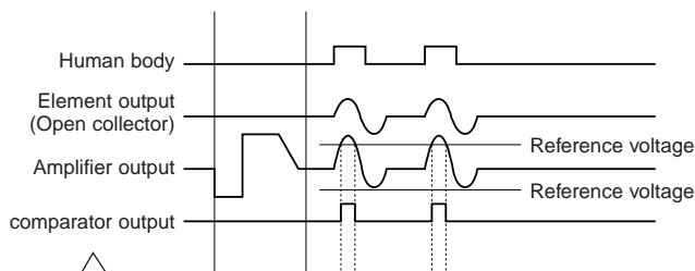
<Timing chart> Standard type
