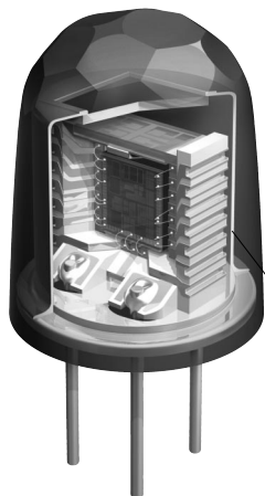
TO5 metal package
