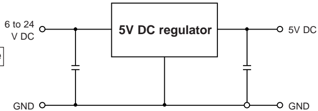
Circuit example
