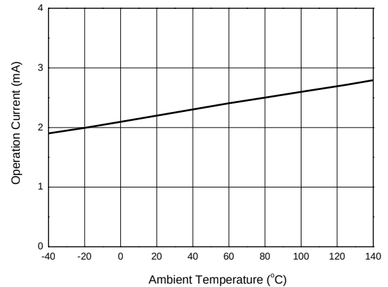
Operation Current vs. Ambient Temperature
