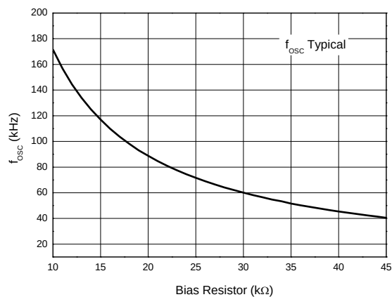
Oscillation Frequency vs. Bias Resistor
