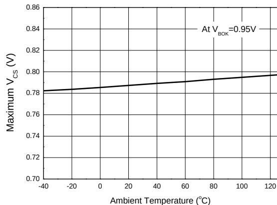
Maximum V_{CS} vs. Ambient Temperature
