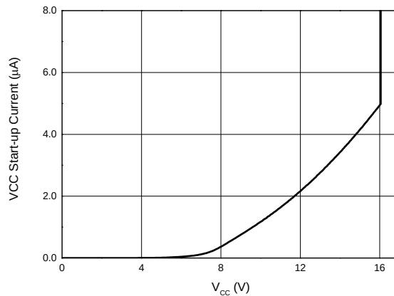
VCC Start-up Current vs. VCC Voltage
