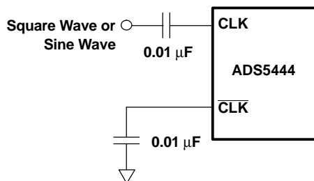
Figure 36. Single-Ended Clock
