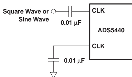
Figure 39. Single-Ended Clock
