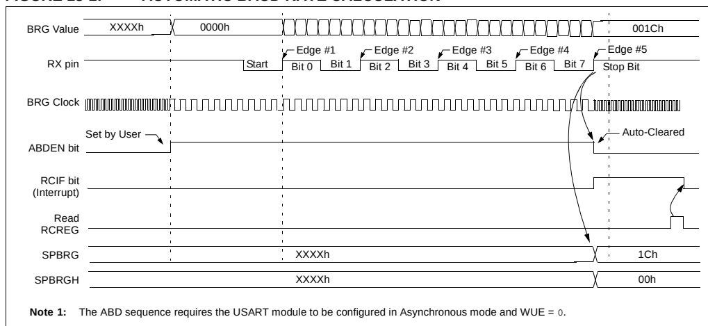
FIGURE 18-1: AUTOMATIC BAUD RATE CALCULATION
