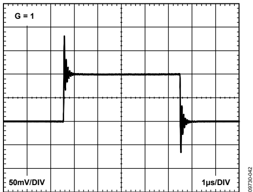
Figure 35. Small Signal Response ( G = 1 ), R_L = 10\text{ k}\Omega , C_L = 100\text{ pF}
