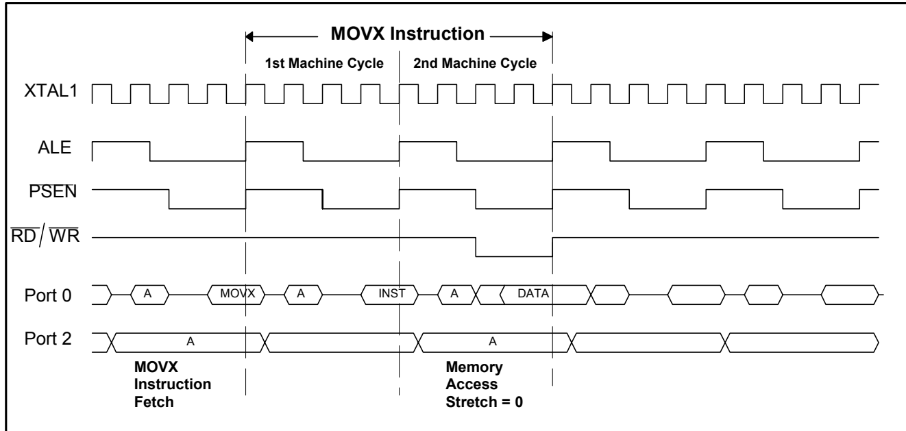
Figure 9. Non-Page Mode, External Data-Memory Access (Stretch = 0, CD1:CD2 = 10)
