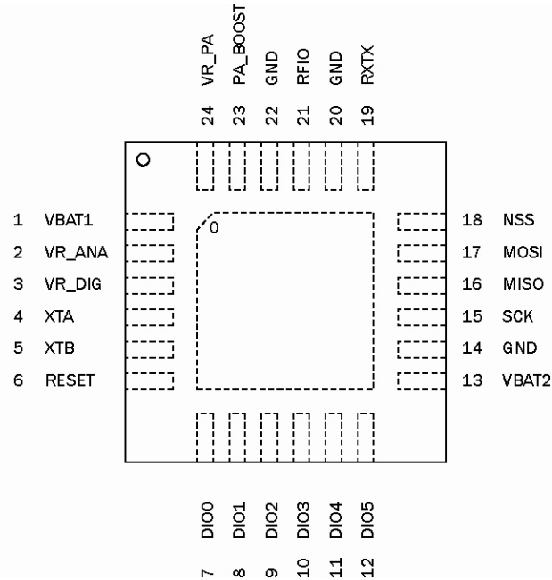
Figure 2. Pin Diagram
