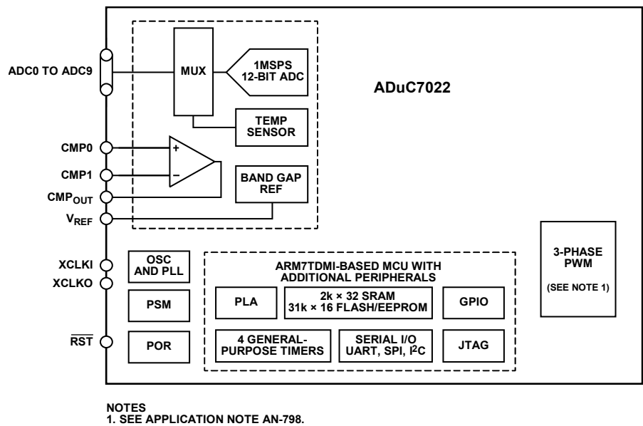
Figure 4. ADuC7022 Functional Block Diagram
