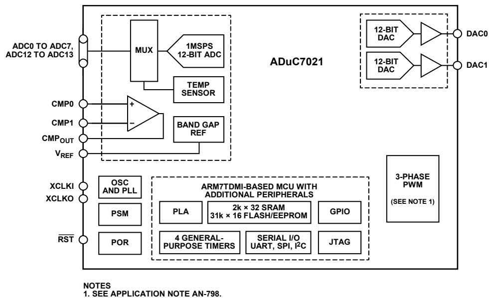
Figure 3. ADuC7021 Functional Block Diagram
