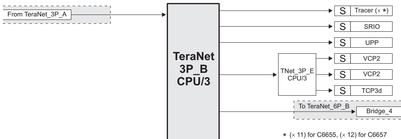
Figure 9-3. TeraNet 3P_B
