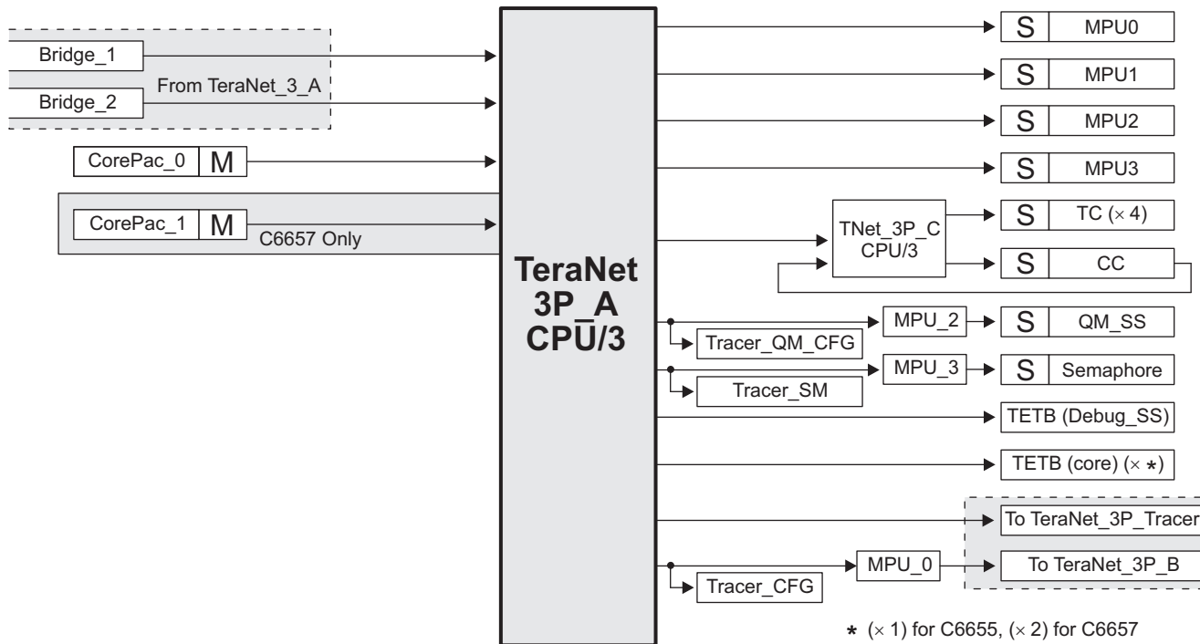
Figure 9-2. TeraNet 3P_A
