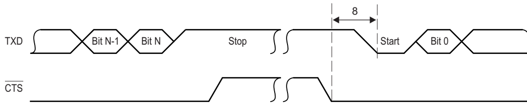
Figure 5-17. UART CTS (Clear-to-Send Input) — Autoflow Timing Waveform
