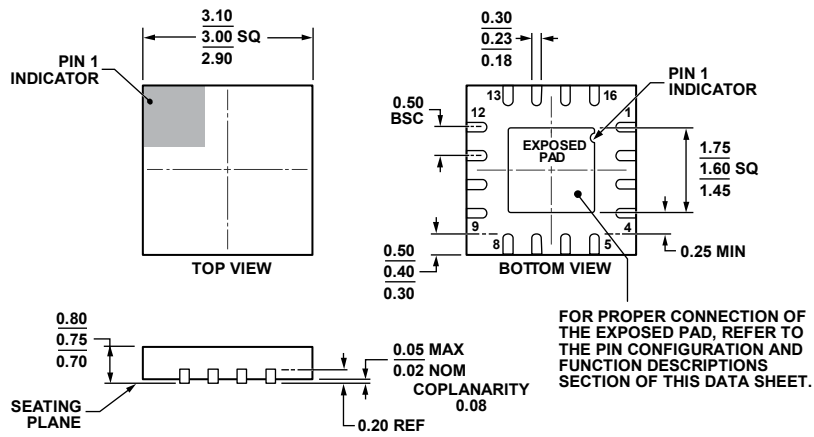
Figure 55. 16-Lead Lead Frame Chip Scale Package [LFCSP_WQ] 3 mm × 3 mm Body, Very Very Thin Quad (CP-16-22)
