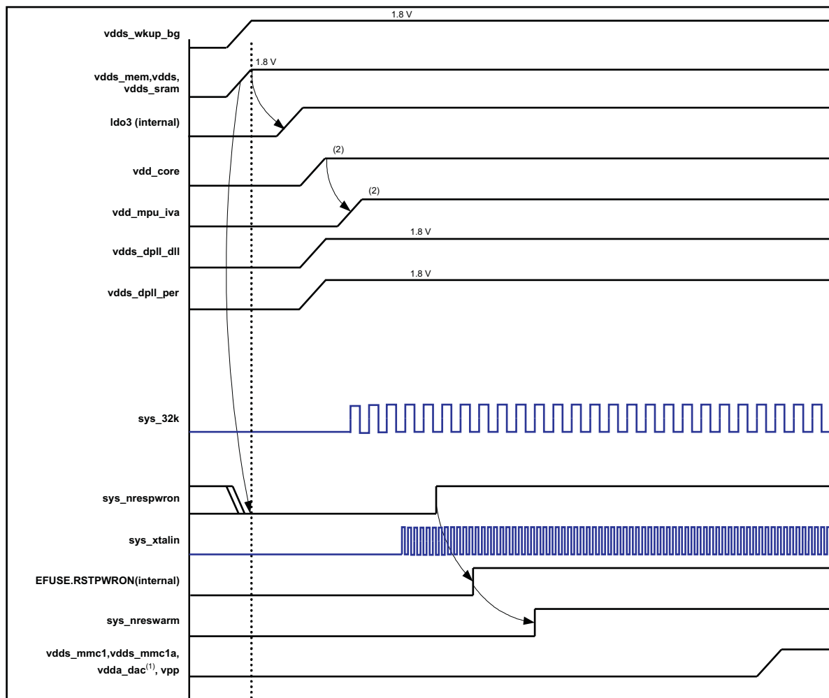
Figure 3-3. Power-up Sequence
