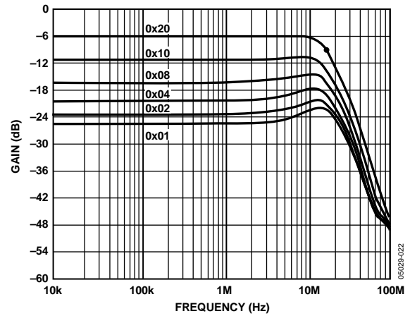
Figure 21. Gain vs. Frequency vs. Code, R_{AB} = 1 k\Omega
