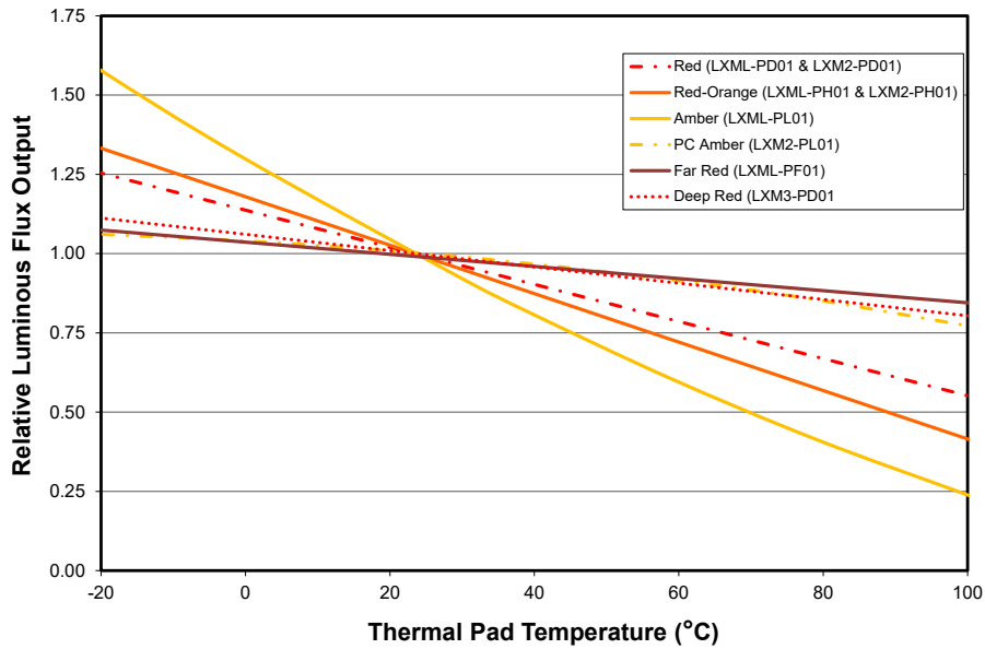
Figure 2b. Typical normalized light output vs. junction temperature for LXML-PF01, LXM3-PD01, LXM2-PD01, LXM2-PH01, LXM2-PL01 at test current.
