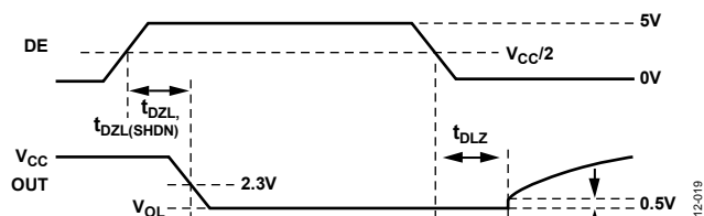
Figure 19. Driver Enable and Disable Times ( t_{DZL} , t_{DLZ} , t_{DZL(SHDN)} )
