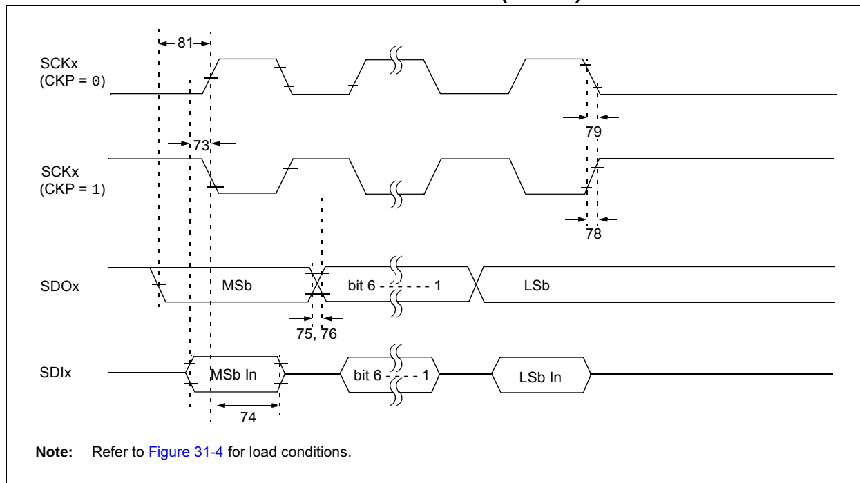
FIGURE 31-13: EXAMPLE SPI MASTER MODE TIMING (CKE = 1)
