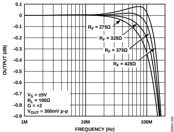
Figure 30. AD9632 0.1 dB Flatness, N Package (for R Package Add 20 \Omega to R_F )
