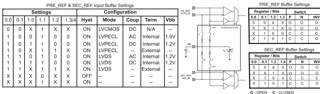
Figure 21. CDCE72010 REF Voltage Biasing Circuitry
