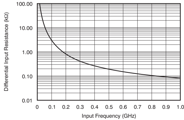
Figure 114. ADC Analog Input Resistance (R IN ) Across Frequency
