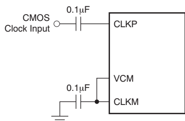
Figure 120. Single-Ended Clock Driving Circuit
