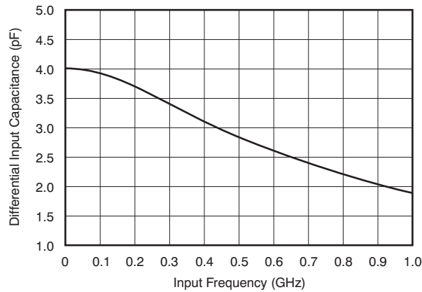
Figure 115. ADC Analog Input Capacitance (C IN ) Across Frequency
