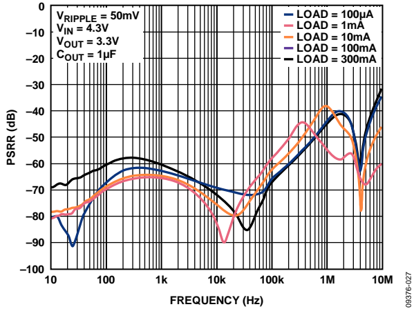
Figure 47. Power Supply Rejection Ratio vs. Frequency, V_{IN} = 4.3\text{ V} , V_{OUTx} = 3.3\text{ V}
