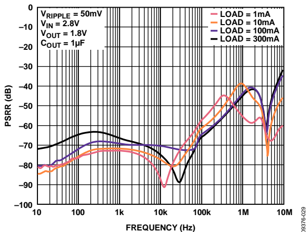
Figure 49. Power Supply Rejection Ratio vs. Frequency, V_{IN} = 2.8\text{ V} , V_{OUTx} = 1.8\text{ V}
