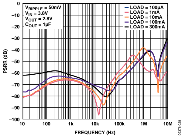
Figure 48. Power Supply Rejection Ratio vs. Frequency, V_{IN} = 3.8\text{ V} , V_{OUTx} = 2.8\text{ V}
