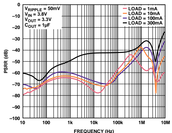
Figure 51. Power Supply Rejection Ratio vs. Frequency, V_{IN} = 3.8\text{ V} , V_{OUTx} = 3.3\text{ V}
