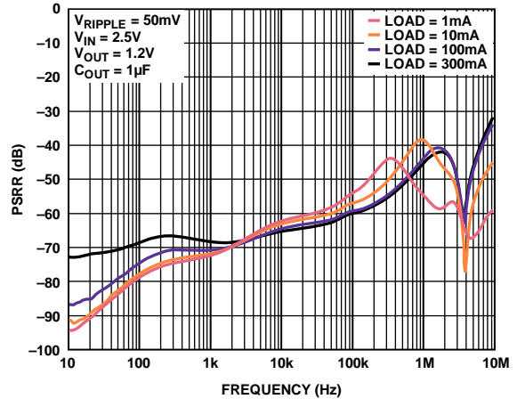
Figure 50. Power Supply Rejection Ratio vs. Frequency, V_{IN} = 2.5\text{ V} , V_{OUTx} = 1.2\text{ V}
