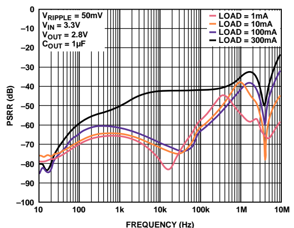
Figure 52. Power Supply Rejection Ratio vs. Frequency, V_{IN} = 3.3\text{ V} , V_{OUTx} = 2.8\text{ V}
