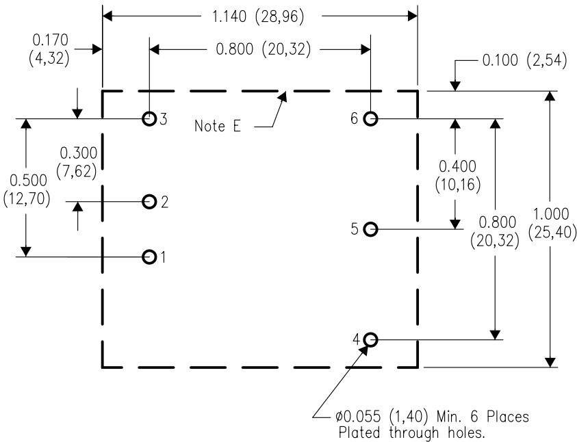
PC LAYOUT
