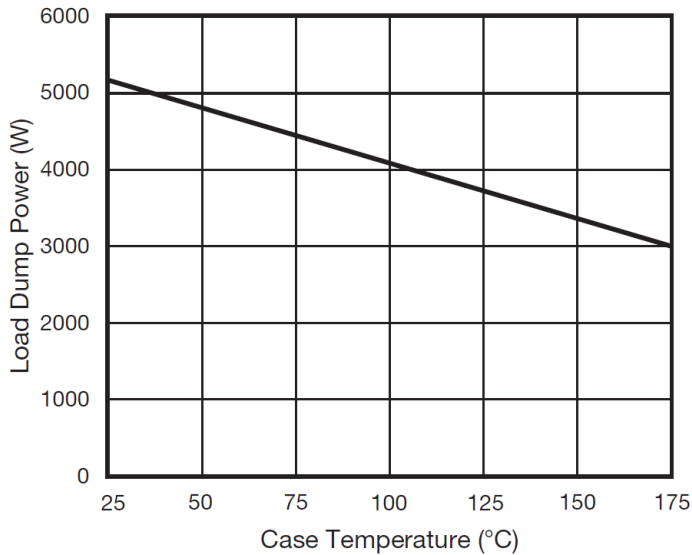
Fig. 2 - Load Dump Power Characteristics (10 ms Exponential Waveform)
