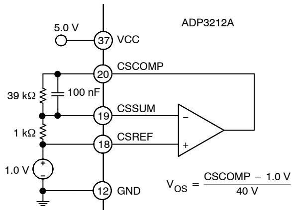
Figure 4. Current Sense Amplifier, V_{OS}
