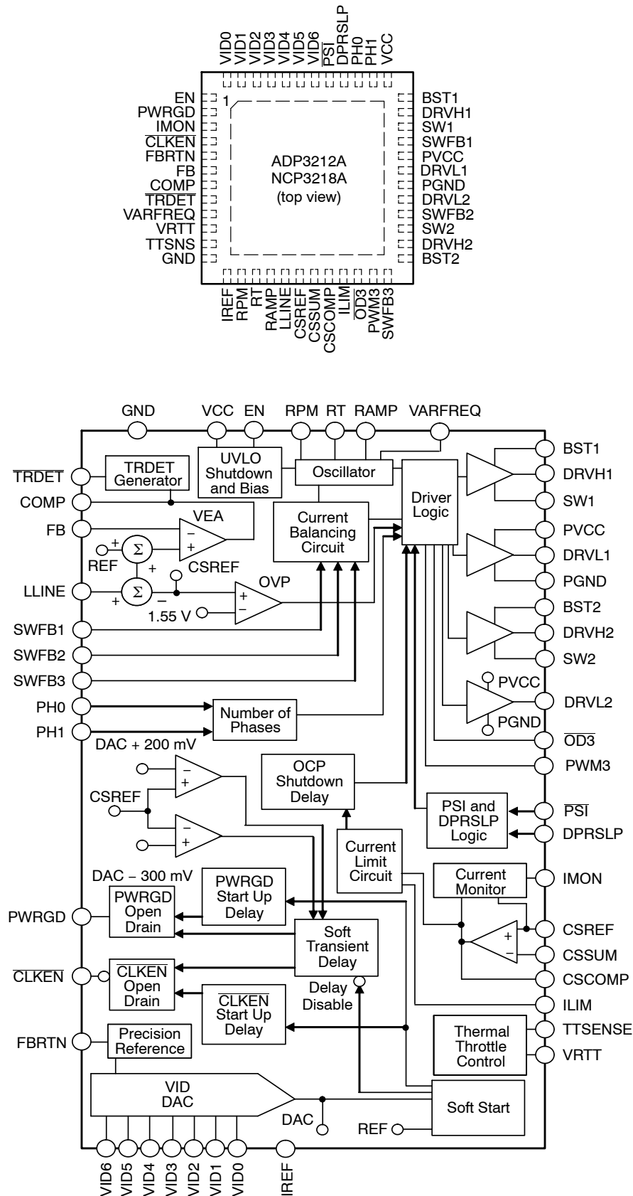
Figure 1. Functional Block Diagram
