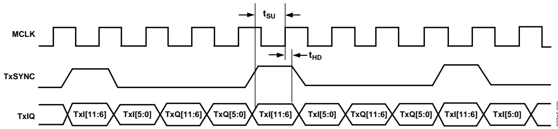
Figure 26. Transmit Timing Diagram
