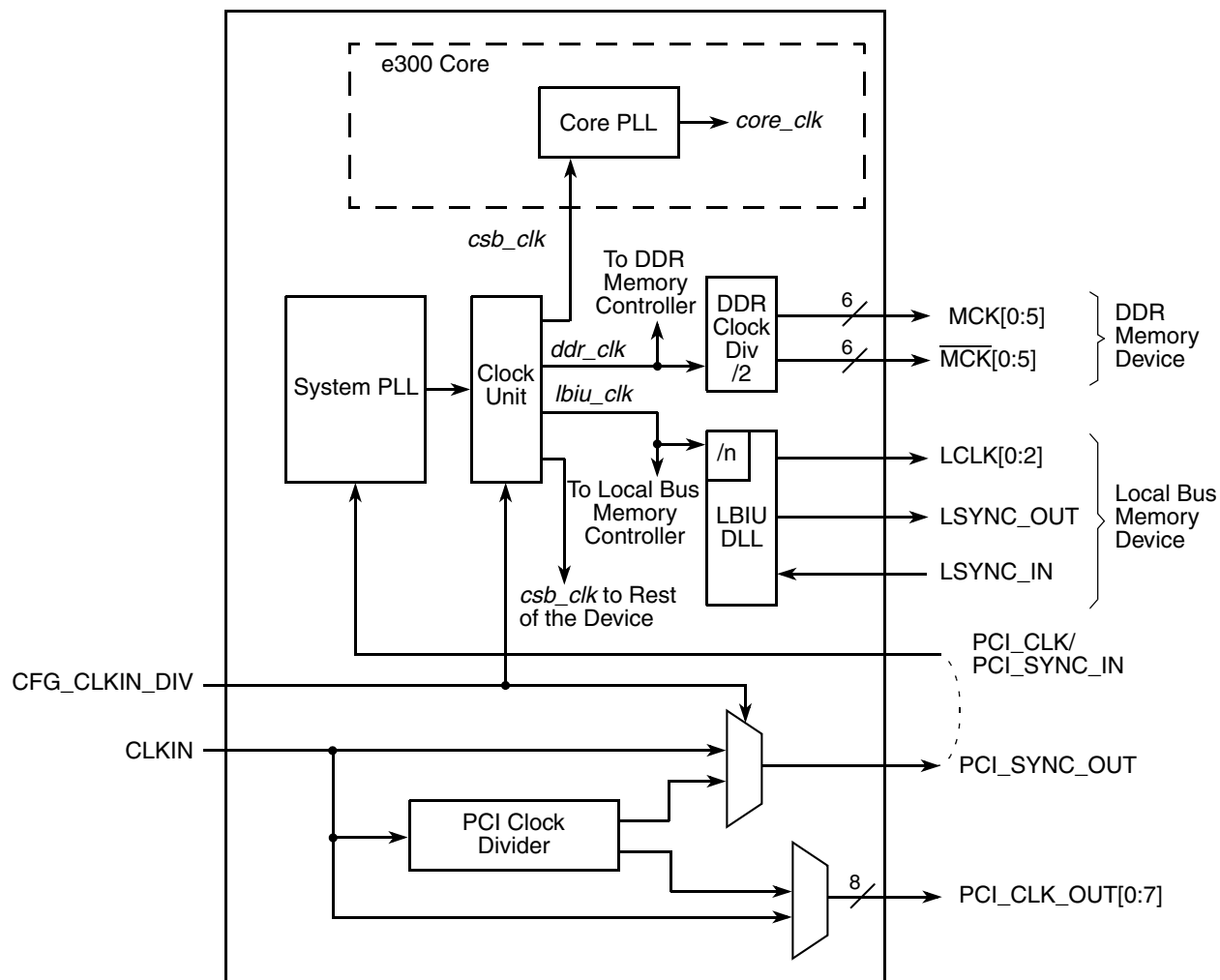
Figure 41. MPC8349EA Clock Subsystem
