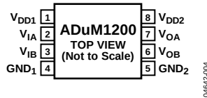
Figure 4. ADuM1200 Pin Configuration
