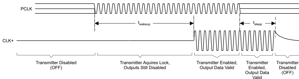
Figure 14. Standby Detection
