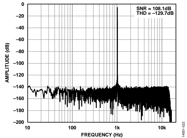
Figure 17. FFT, Eco Mode, Wideband Filter, -6 dBFS
