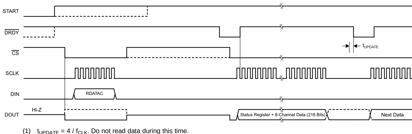
Figure 46. RDATA Usage
