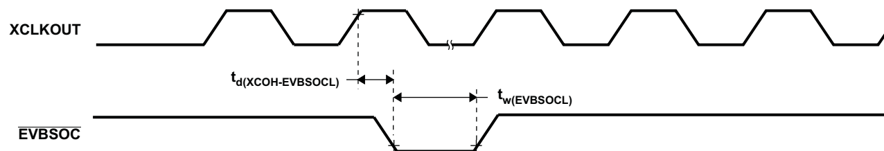
Figure 5-18. EVBSOC Timing
