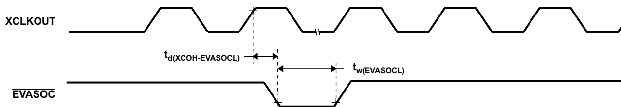
Figure 5-17. EVASOC Timing
