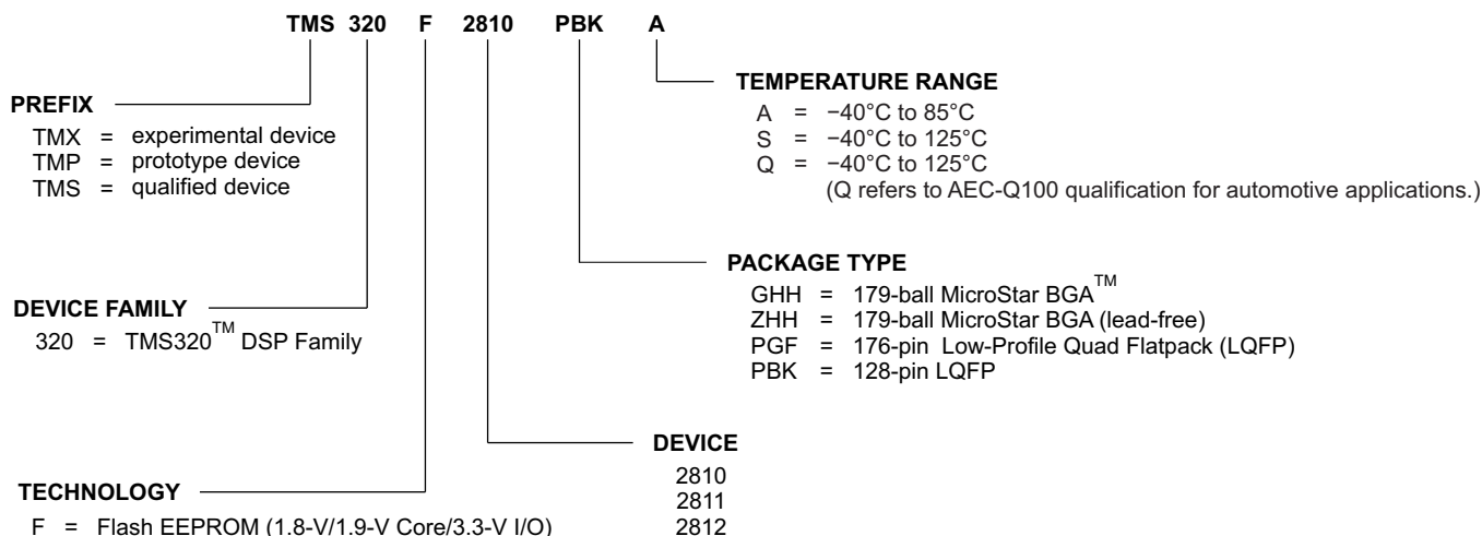
Figure 8-1. TMS320F281x Device Nomenclature
