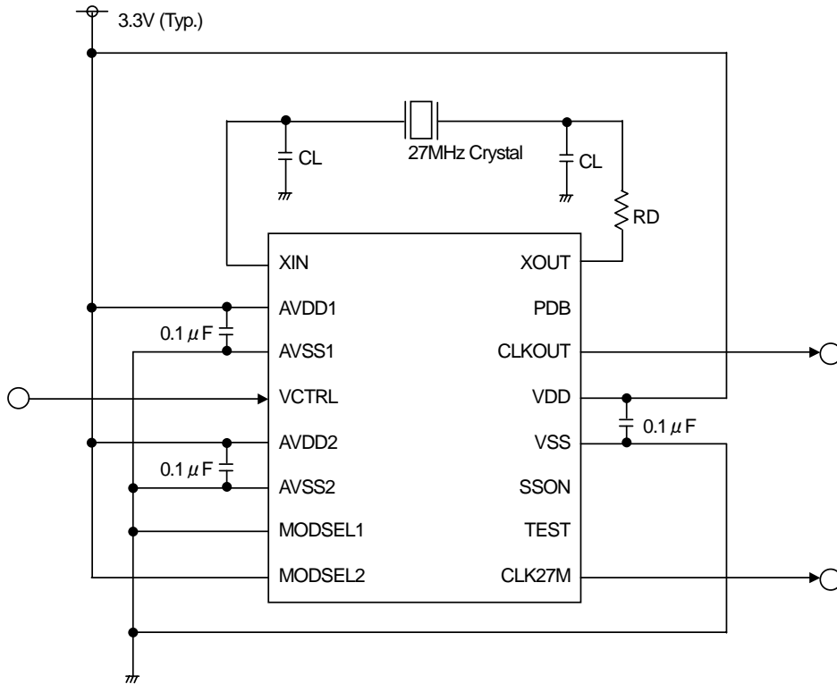
Figure 48. Modulation Rate \pm 0.75\% setting Typical Application Circuit
