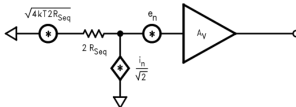
Figure 56. Noise Model with R_f || R_g = R_{seq}
