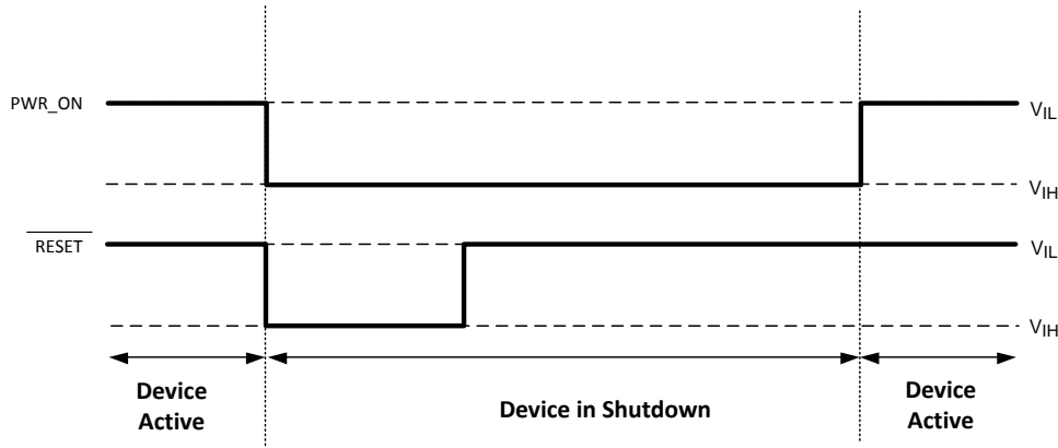
Figure 50. I 2 C Reset Timing Diagram
