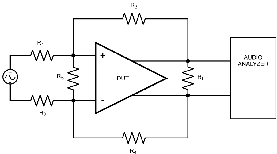
Figure 54. THD+N and IMD Distortion Test Circuit
